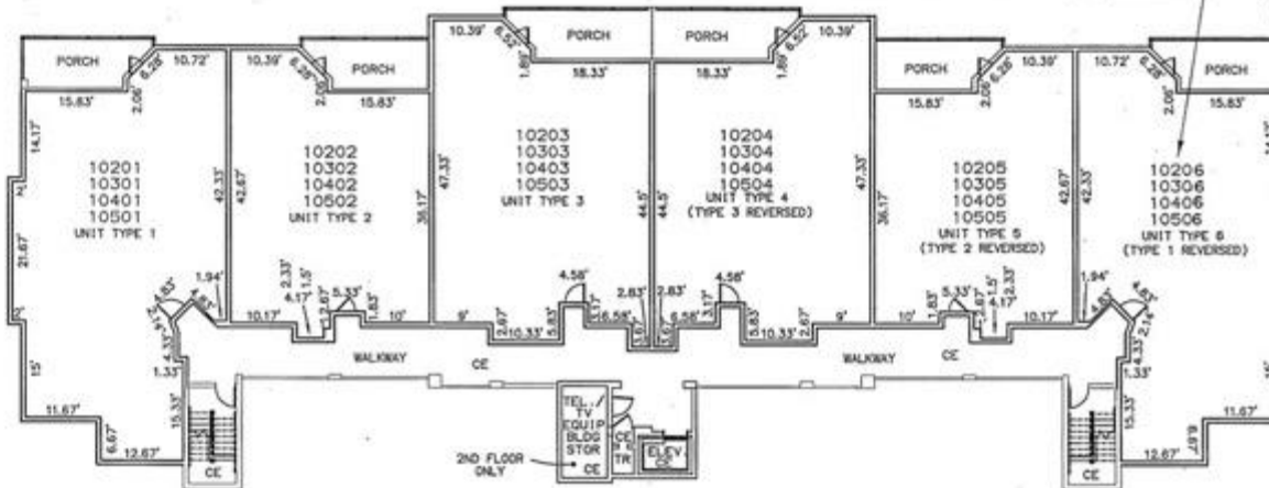
SECOND THROUGH FIFTH FLOOR PLAN
